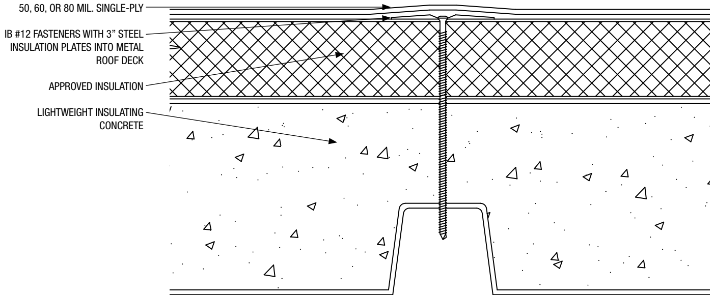
50 60 80 FA-RI-LWIC (Lightweight Concrete) FastSpec™
