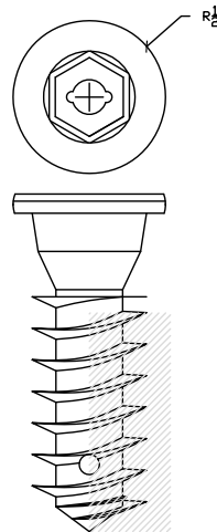
NTB Fastener
